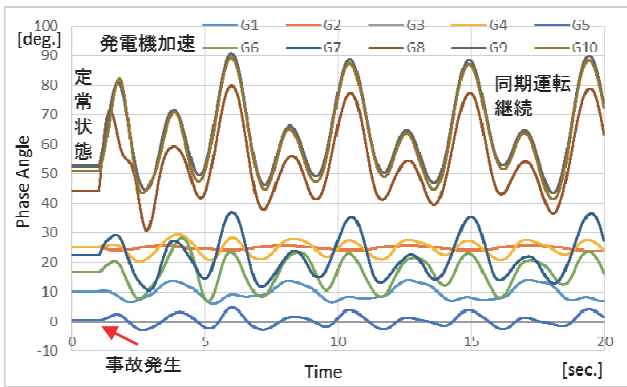
Fig. 6 Phase angle of generators (Ref. G3).
