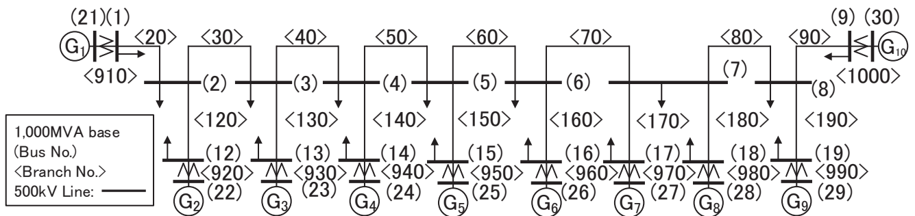
Fig. 8 Western 10 machines - power system model (WEST10).
