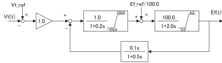
Fig. 2 Block diagram of automatic voltage regulator in the standard power system models.
