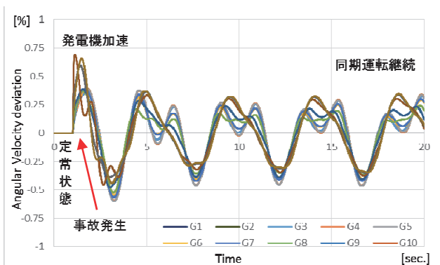
Fig. 7 Angular velocity deviation of generators.
