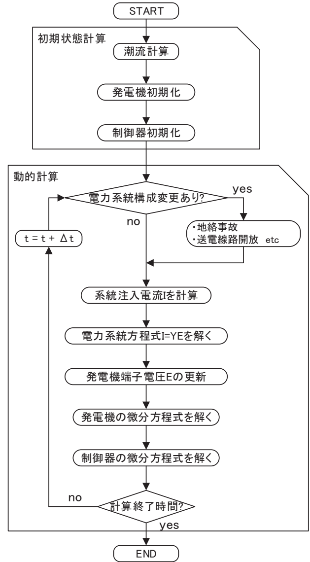
Fig. 1 Flow chart of transient stability calculation.
